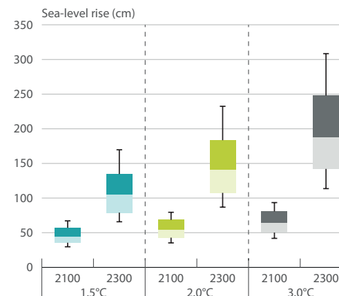
Long term sea level rise Relative to 1986-2005
